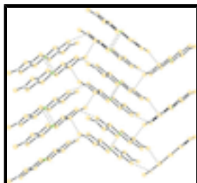
Fig. 2. Two-dimensional supramolecular structure of [\text{Ni}(\text{dmit})_2]^- anions through \text{S}\cdots\text{S} and \text{Ni}\cdots\text{S} contacts. Dashed lines indicate weak interactions.
